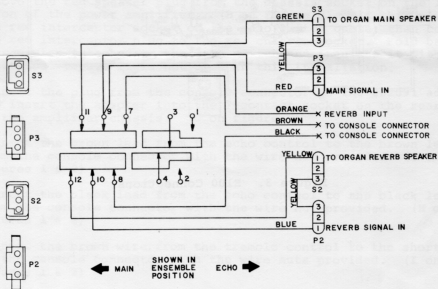
Figure 4. Schematic, Echo Control 011882 (Plugs and Sockets Shown from Wire End)
