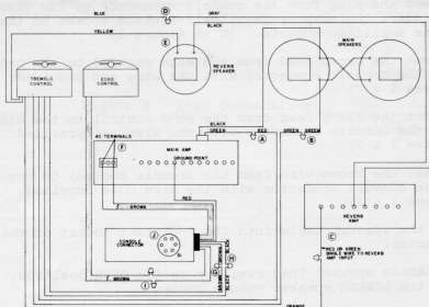
Figure 2. M100 Connections
