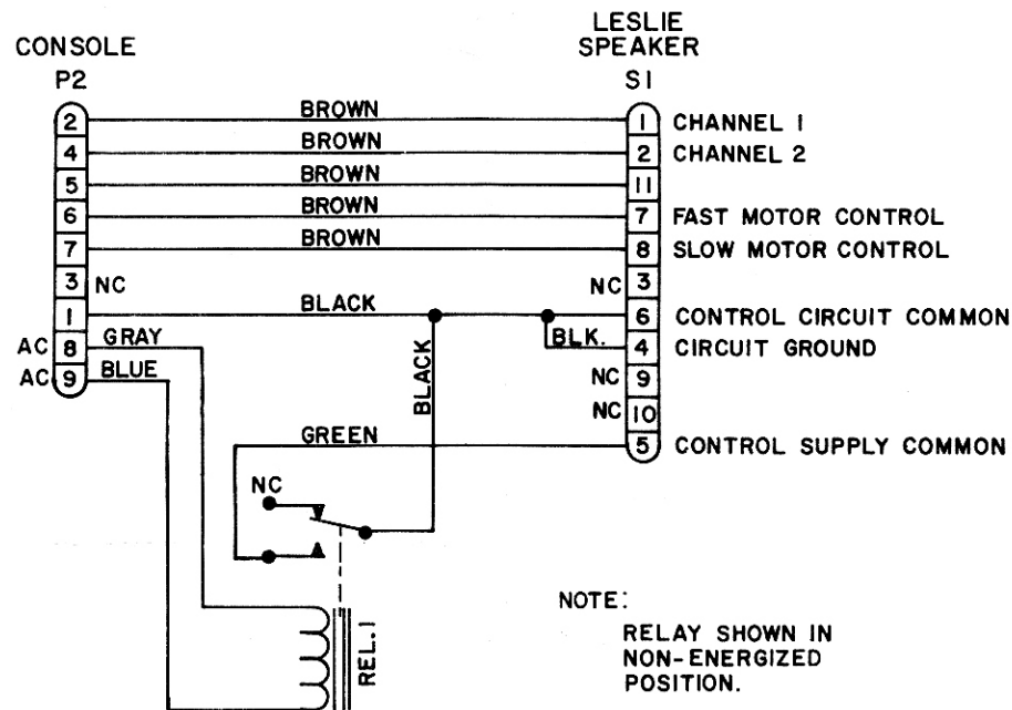
Figure 2. Schematic, Adapter 138158
