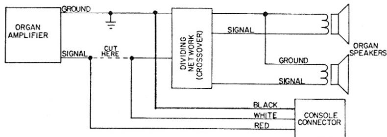
Fig. 4. Single-Channel Organs with crossover network and several speakers
