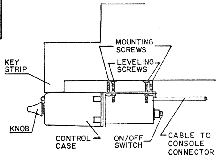
Figure 3. Control Mounted on Organ
