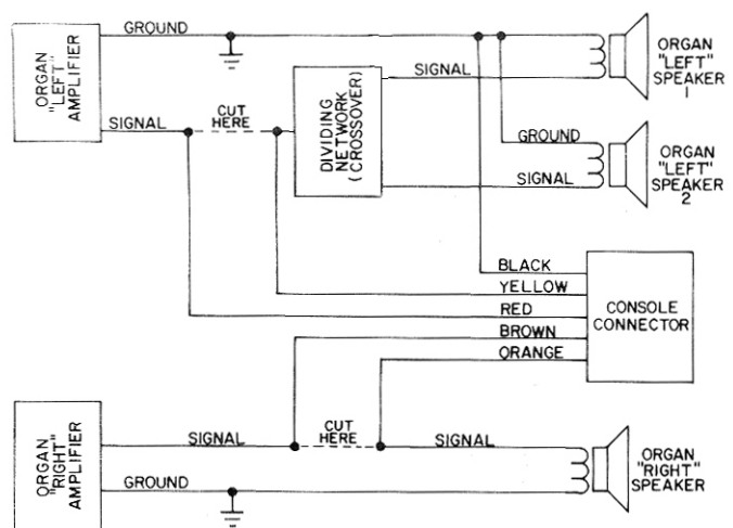
Figure 4. Interconnections When Dividing Network is Present
