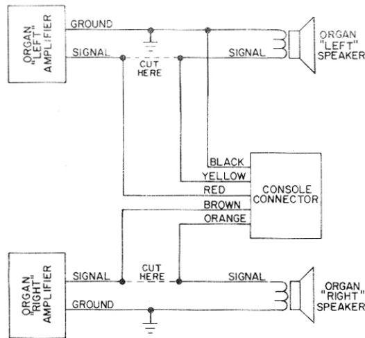
Figure 3. Interconnections, Two-speaker Organ
