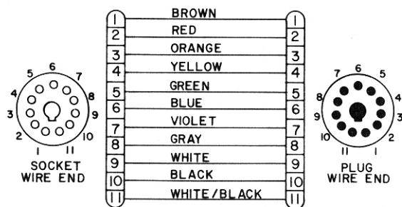
Figure 3. Schematic, Cable Assembly
