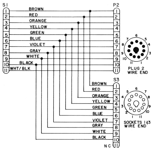
Figure 2. Schematic, Y Adapter
