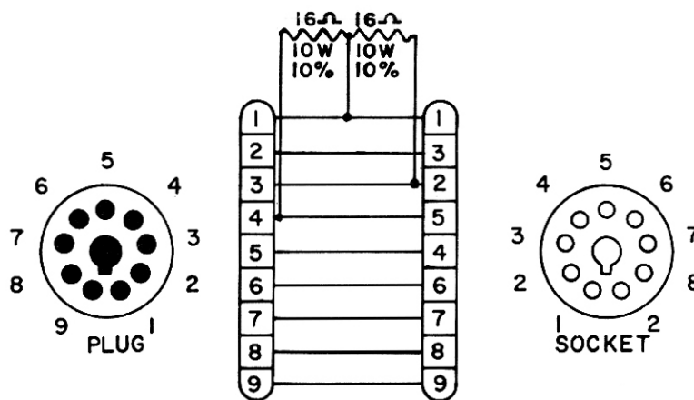
SCHEMATIC: 107320 CONSOLE CONNECTOR
