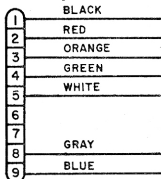
Figure 2. 027276 Adapter
