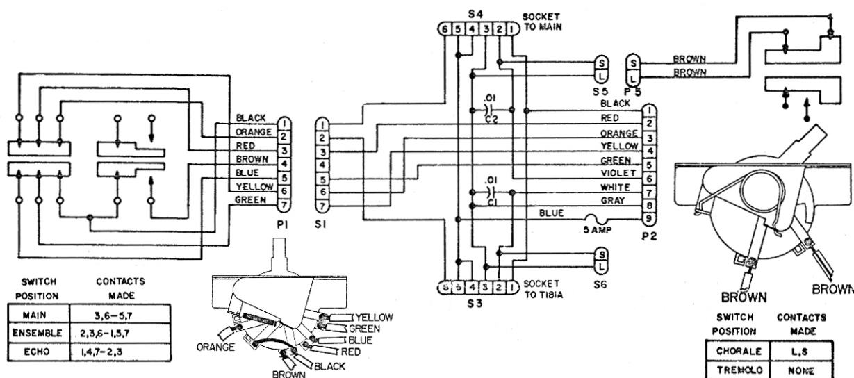
Figure 1. Schematic, 062042 Console Connector with Controls
