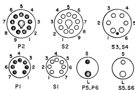
Figure 3. Plug and Socket Base Diagram
