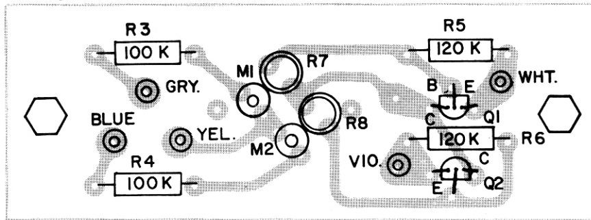
Circuit Board Assembly 063818
