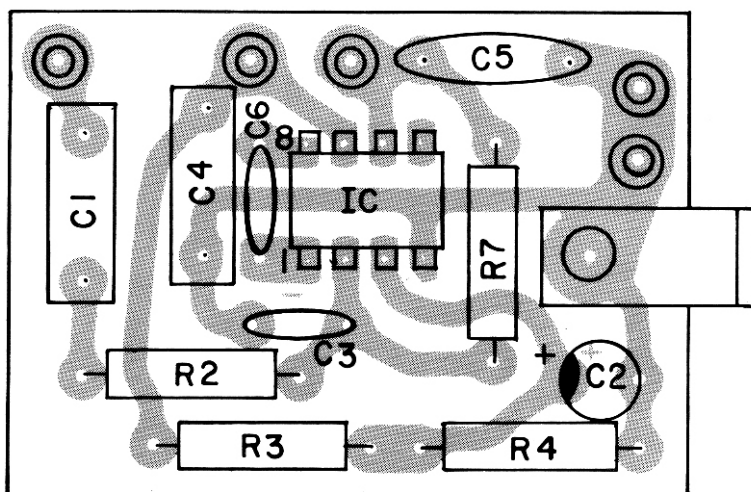
Figure 5. Circuit Board Assembly 112660
