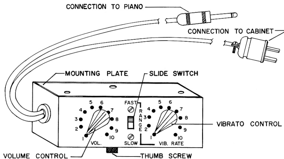
Figure 1. Control Assembly 112670
