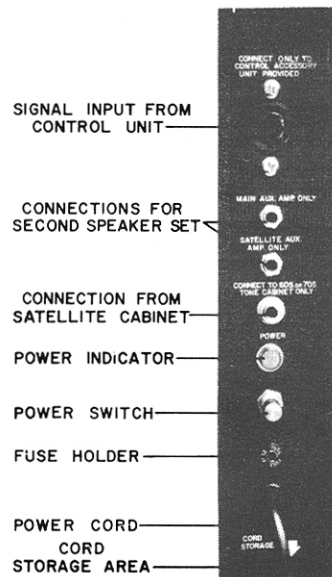
Figure 2. Power Supply Panel, Showing Connections
