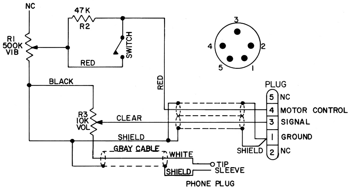
Figure 4. Schematic, Control 110750
