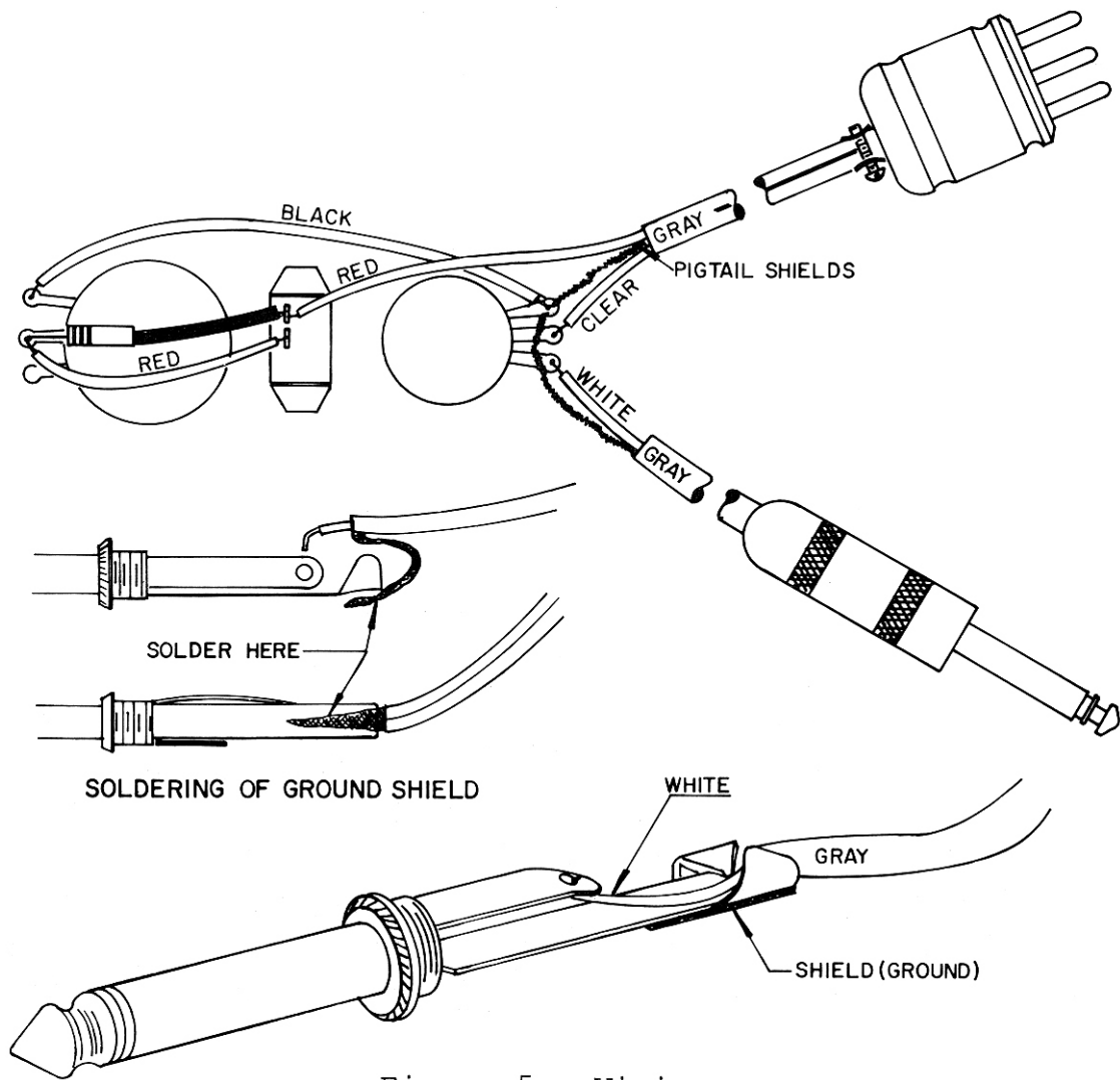
Figure 5. Wiring
