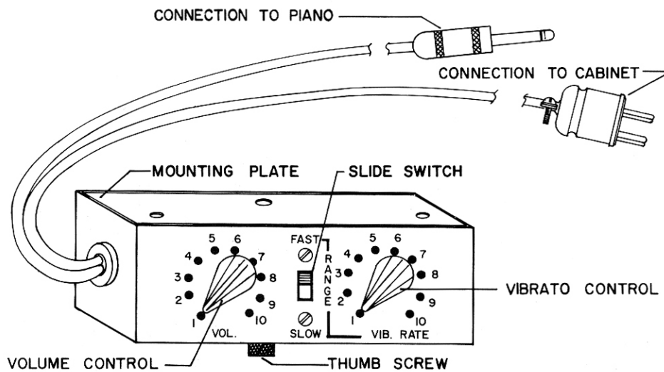
Figure 1. Control Assembly 110750
